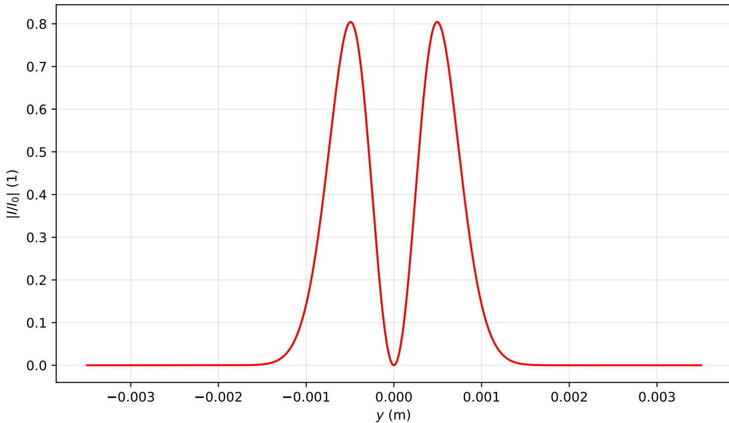
Intensity profile I(x=0, y, z=0.080)/I_0 , P_{in}=7.0P_{cr} , artificial time
